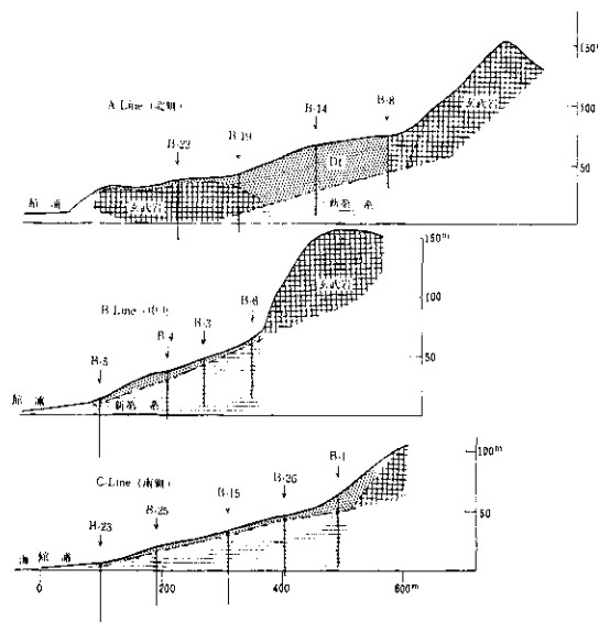
図-16 佳路地区の地下構造断面 (H : V = 1 : 2) Fig. 16 Assumed diagrams of underground profiles at the Garo landslide area.
