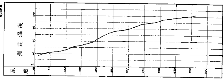
図5 2号試験井の温度検層図 Fig. 5. Temperature log of the test well No. 2.
