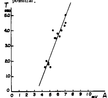
Fig.6 Relation between the periods of electrode vibration in water and the amplitude of earth-current potential.
