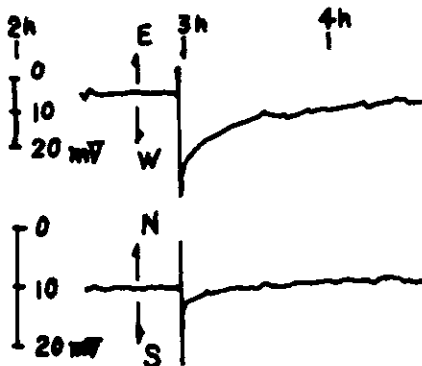
Fig.11 Anomalous change in earth-current potential gradient at the time of an earthquake on Nov 23 1966 at Mt. Minakami.
