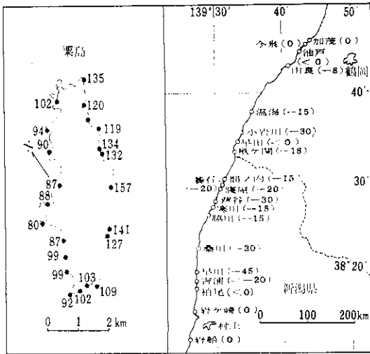
Fig. 4. The vertical movement of earth's crust in cm. ○: subsidence, ● up heaval. Reprinted from the reference 2), 3) .
